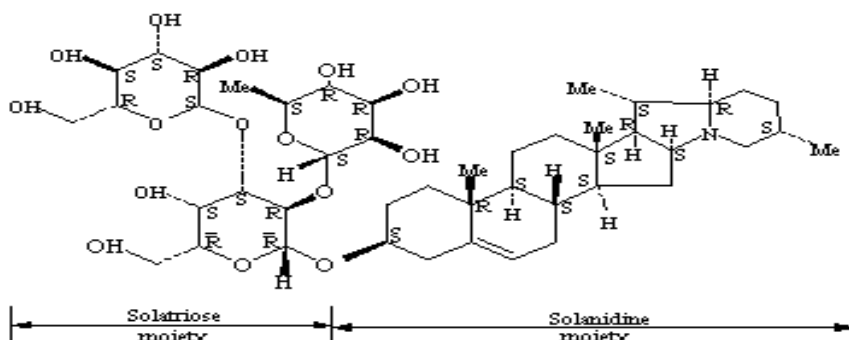
Fig. 1: Solanine structure
